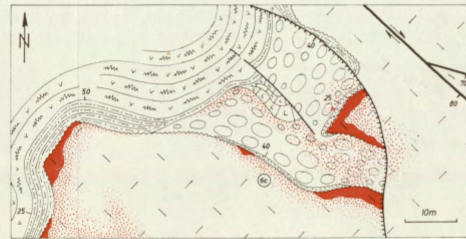
C Rudno telo Talnina (5c) nad 5. obzorjem Talnina ore body (5c) above the 5th level
