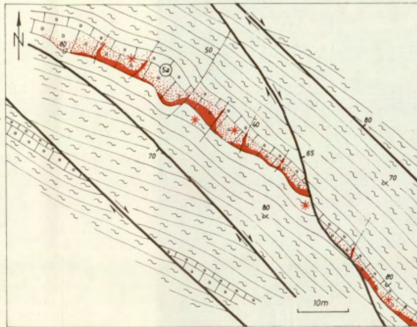
B Rudno telo Ruda (5a) nad 12. obzorjem Ruda ore body (5a) above the 12th level
