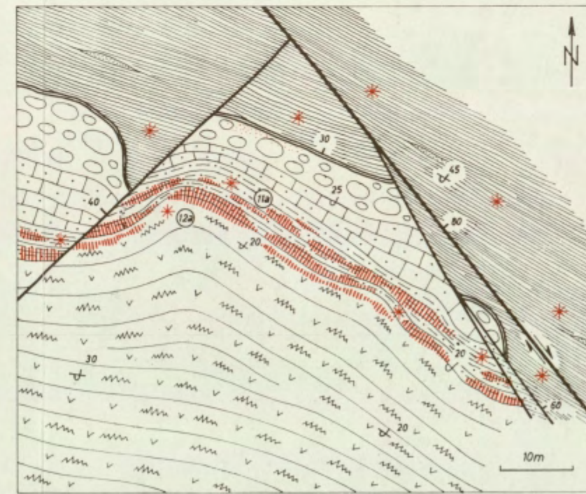
F Rudno telo Kropač (11a in 12a) nad 1. obzorjem Kropač ore body (11a and 12a) above 1st level
